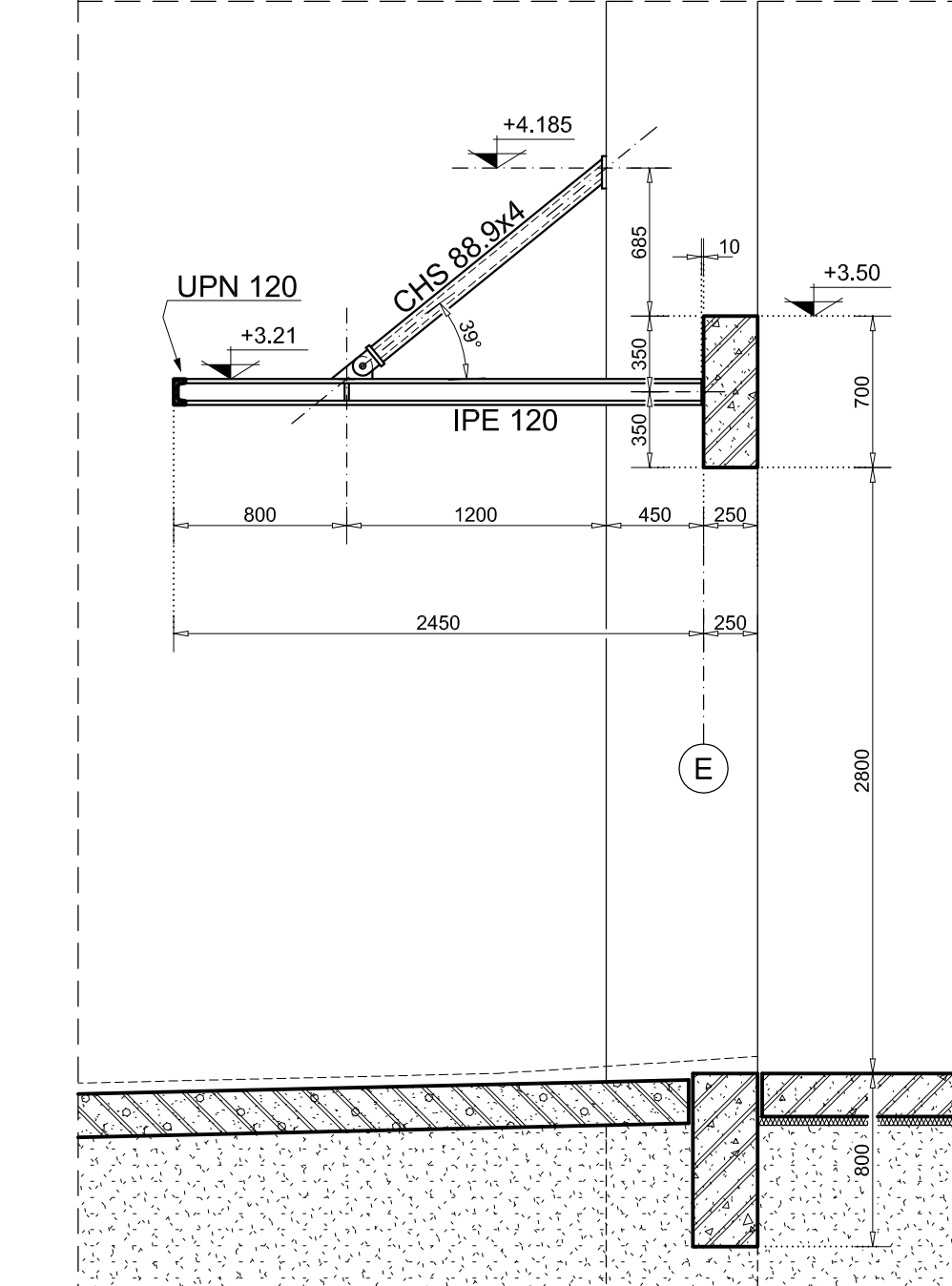
Τομή [E-E]
